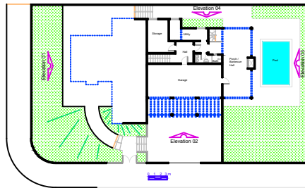
Lower Floor Plan A = 123,64 m 2
