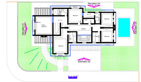
Second Floor Plan A = 208,40 m 2
