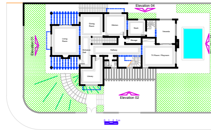
First Floor Plan A = 208,24 m 2
